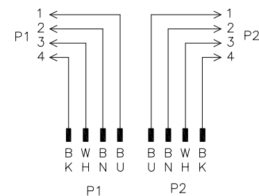
WIRING DIAGRAM
